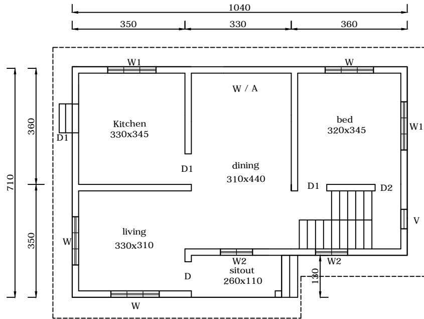
GROUND FLOOR PLAN 745 sqft
